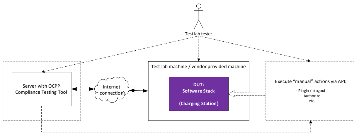
Figure 4: Test setup for testing Charging Station software stacks
