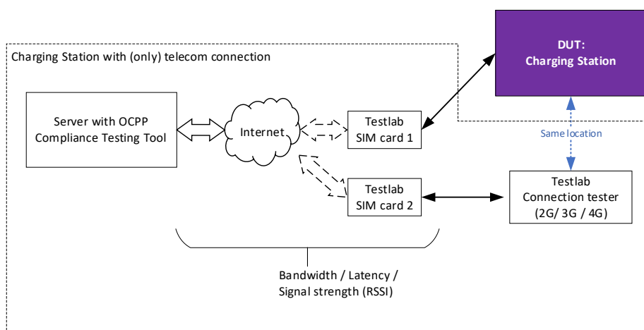
Figure 3: Test setup for a Charging Station with (only) telecom connection
