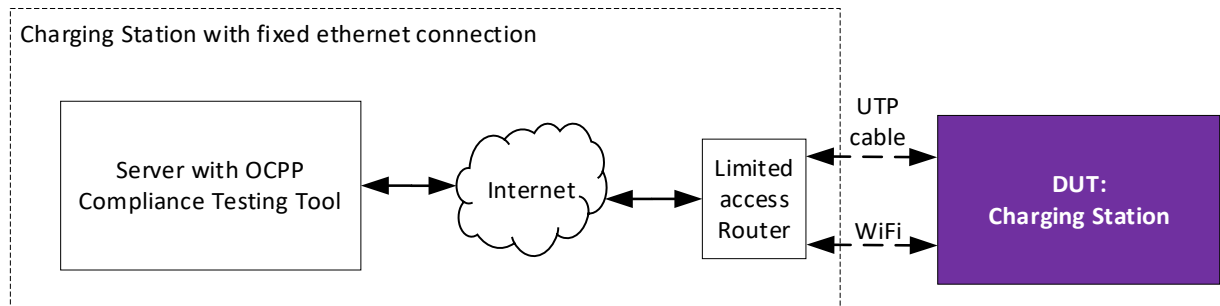
Figure 2: Test setup for a Charging Station with fixed ethernet connection
